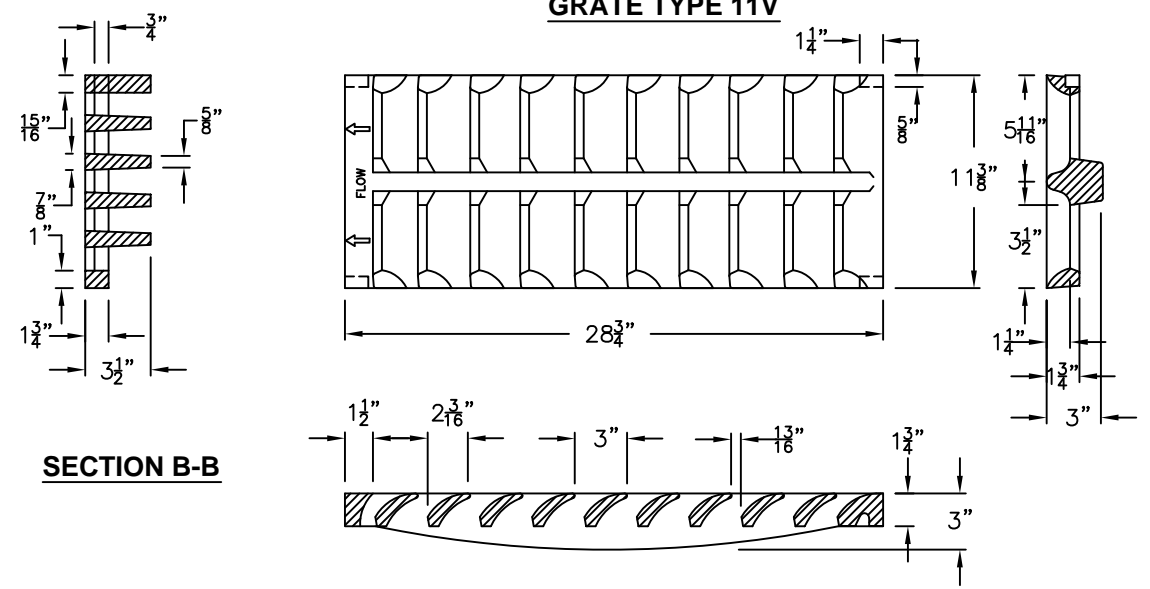
GRATE TYPE 11V
