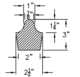
MIDDLE RIB DETAIL
