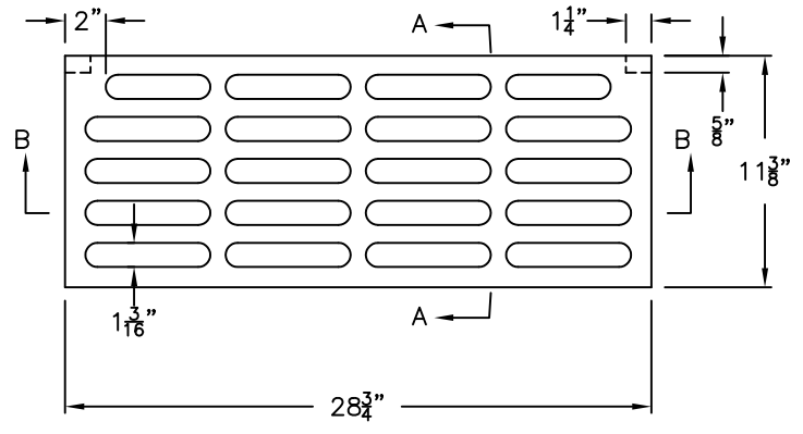
GRATE TYPE 11
