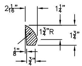
SIDE RIB DETAIL
