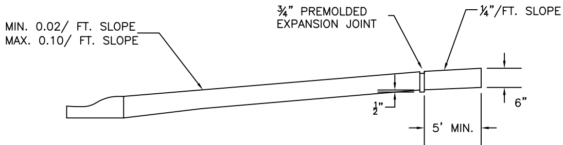
TYPICAL SECTION
